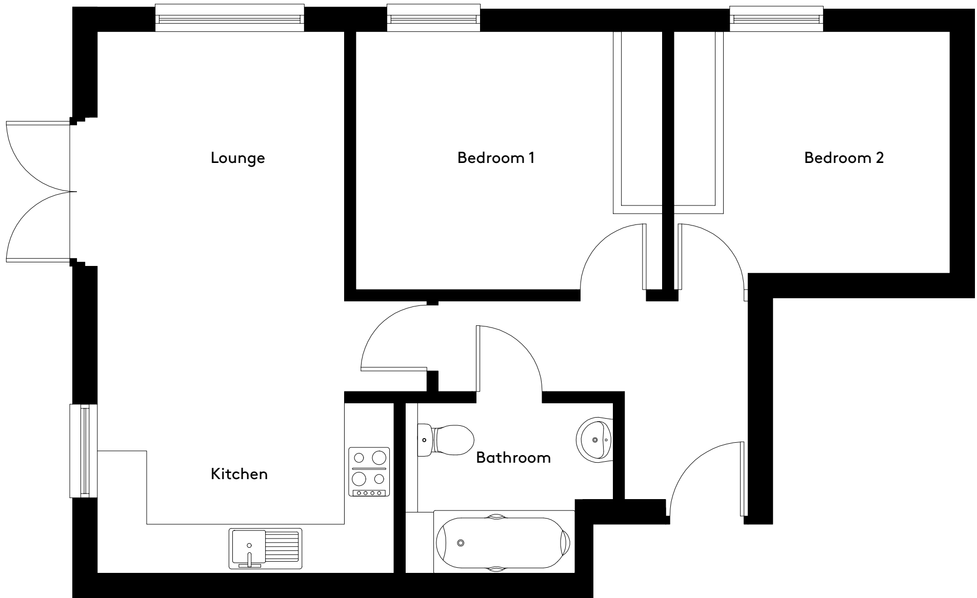
2 Park Lodge Ground floor
